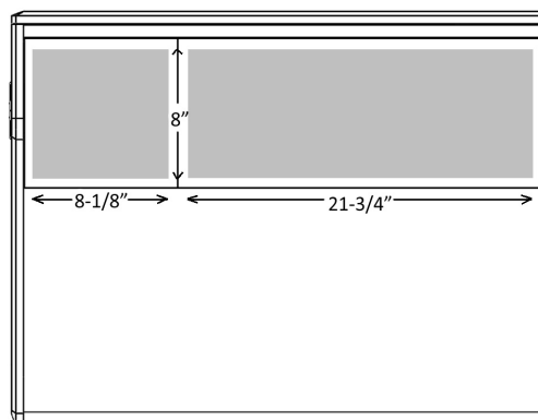
FF - Flat Top Configuration
