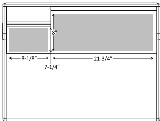
WF - Wedge/Flat Top Configuration
